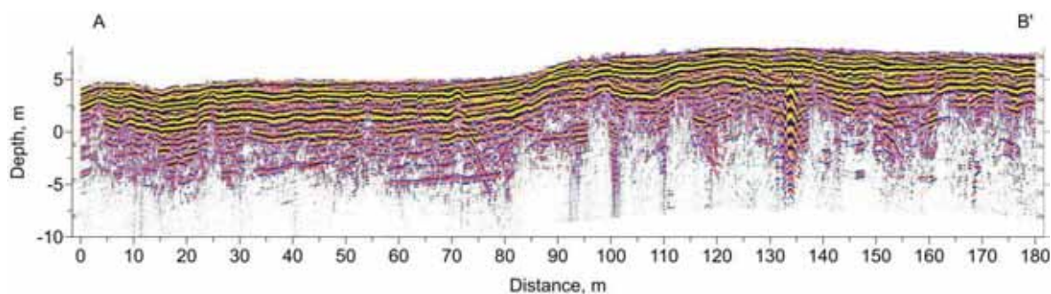
Fig. 7. Ground penetrating radar data along the AB' profile (Fig. 1)
