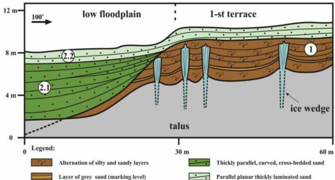
Fig. 3. Geological scheme of Samoylov Island coastline structure
